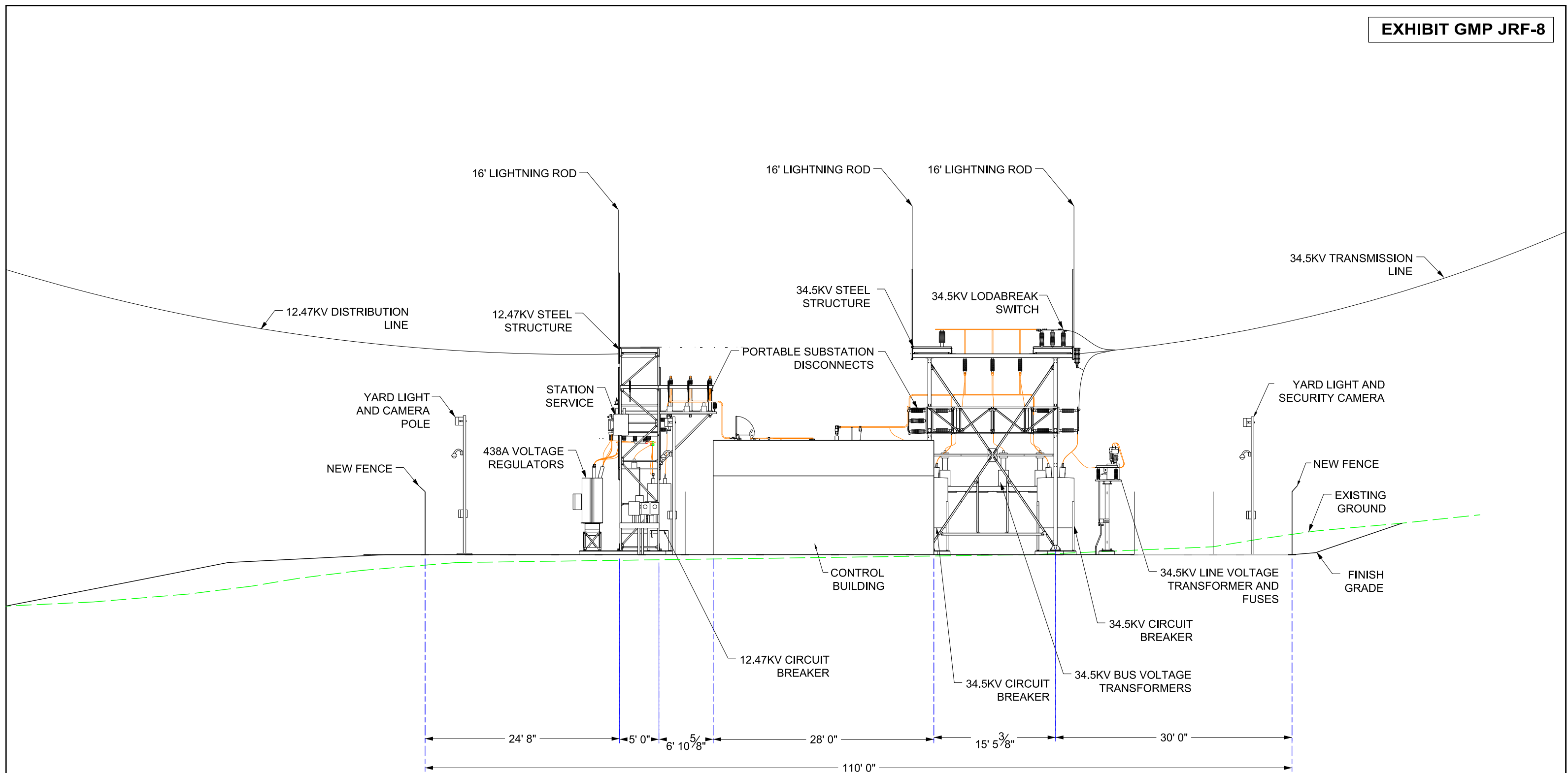
SOUTH ELEVATION - DD (FACING NORTH)
