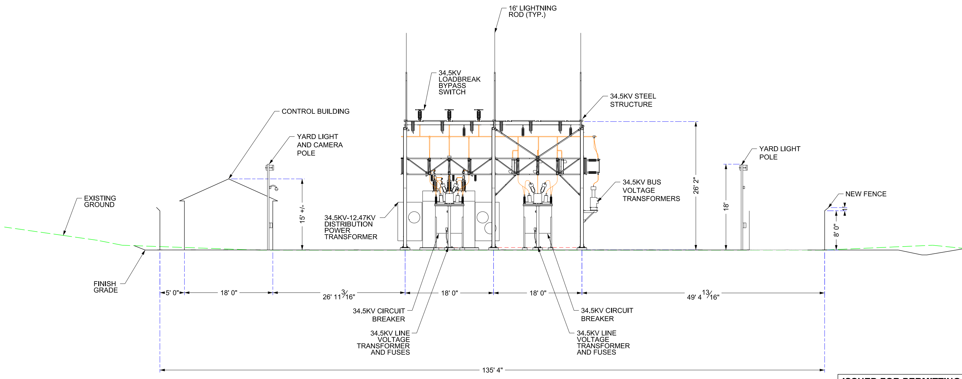
EAST ELEVATION - BB (Facing West)
