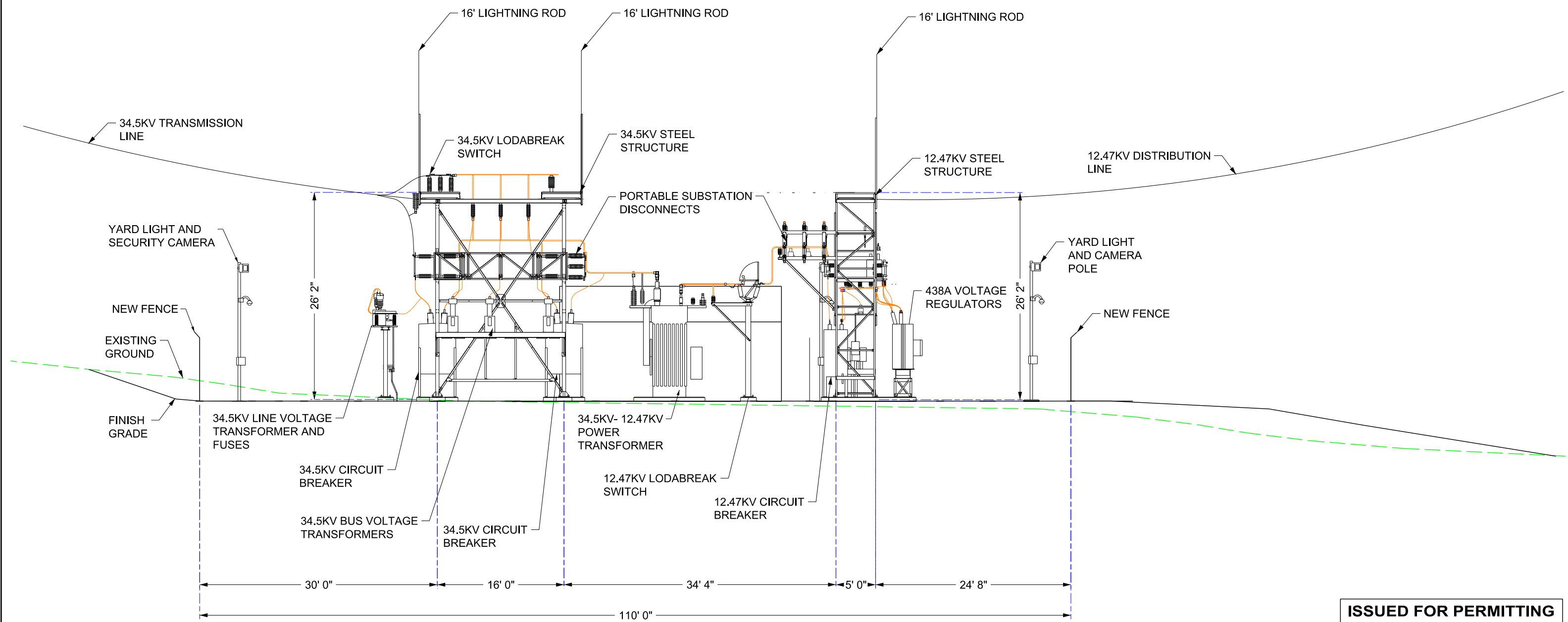
NORTH ELEVATION - AA (FACING SOUTH)
