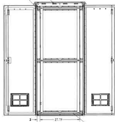
SECTION AD-AD SCALE 1:12
