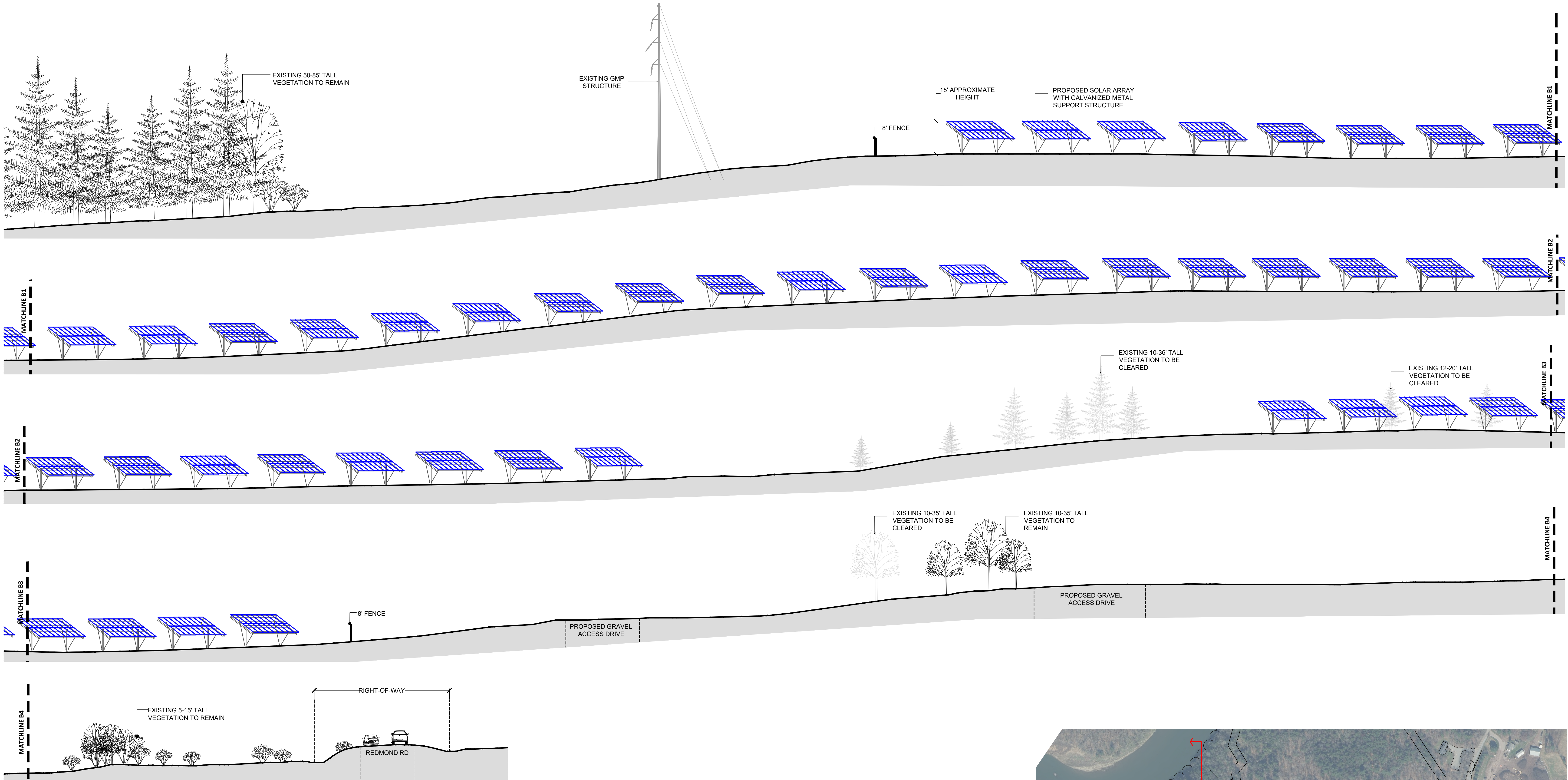
B SECTION B: LOOKING EAST SCALE 1" = 20'
