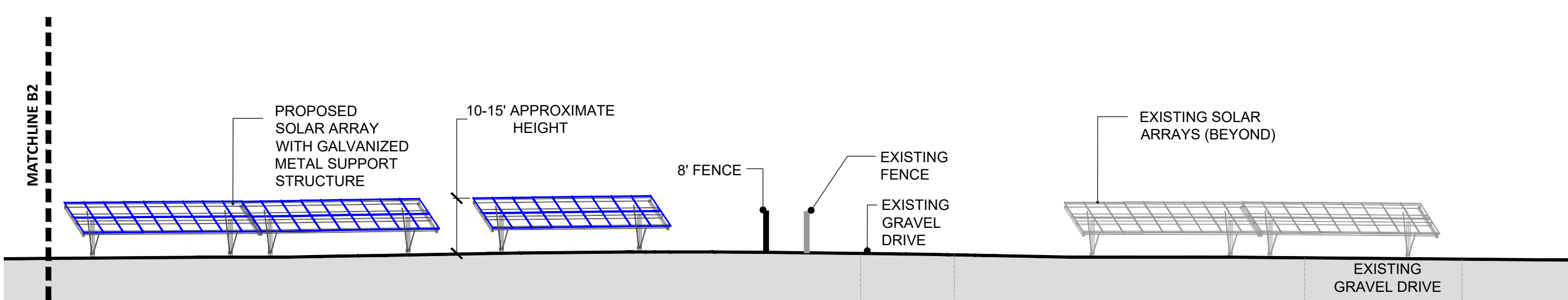
2 SECTION B2: LOOKING NORTH SCALE 1" = 20'
