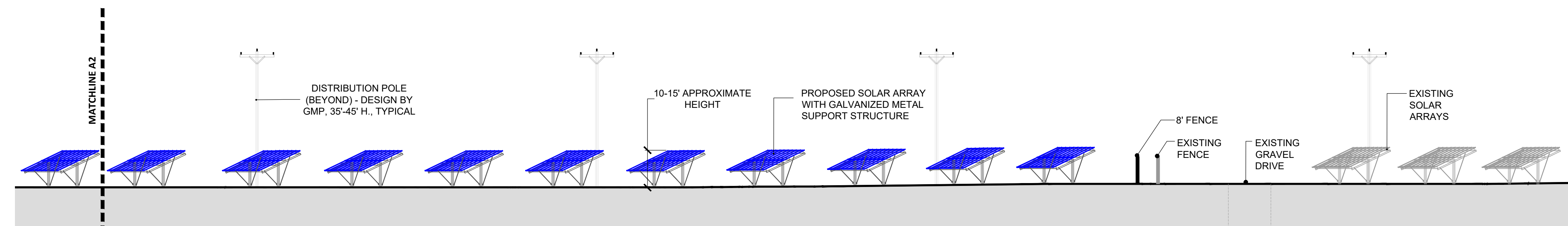
1 SECTION A2: LOOKING WEST SCALE 1" = 20'
