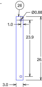
Seismic Provision Detail
