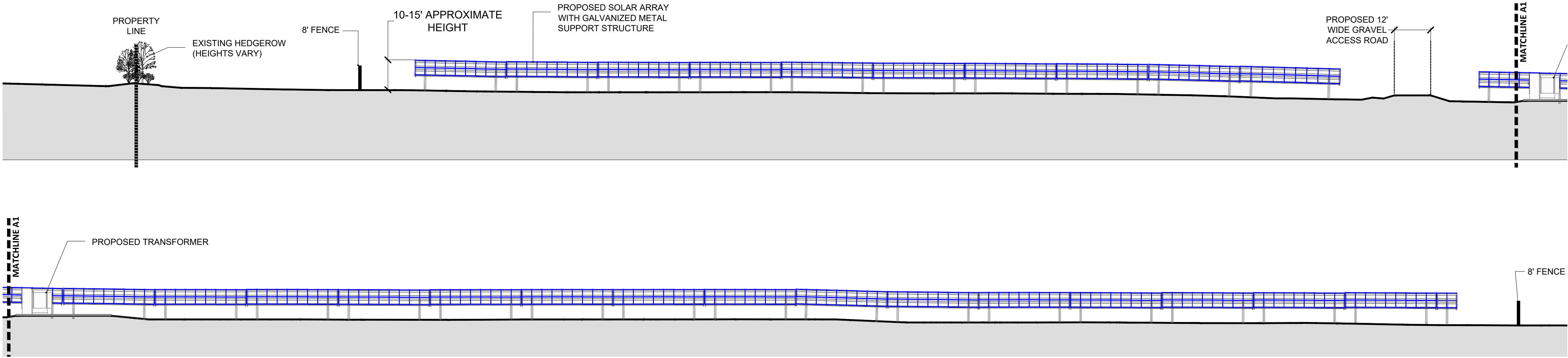
1 SECTION A: LOOKING EAST SCALE 1" = 20'
