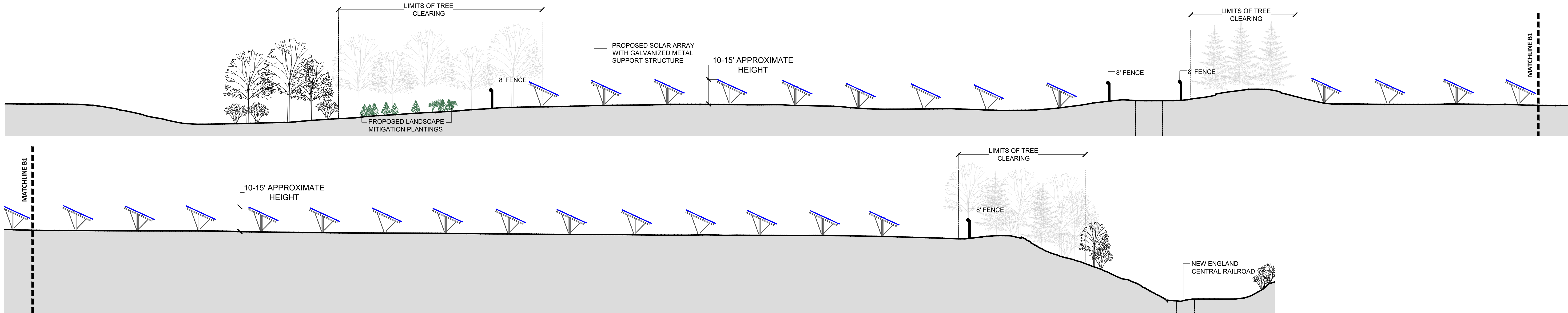
2 SECTION B: LOOKING EAST SCALE 1" = 20'
