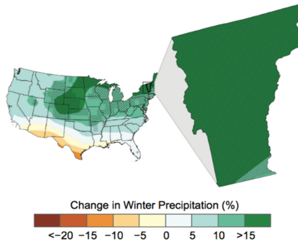
Figure 5: Projected change in winter precipitation (%) by the middle of the 21st century compared to the late 20th century under a higher emissions pathway. Hatching represents areas where the majority of climate models indicate a statistically significant change. Vermont is part of a large area of the Northeast that is expected to experience increases in winter precipitation. Source: CICS-NC and NOAA NCEI.
