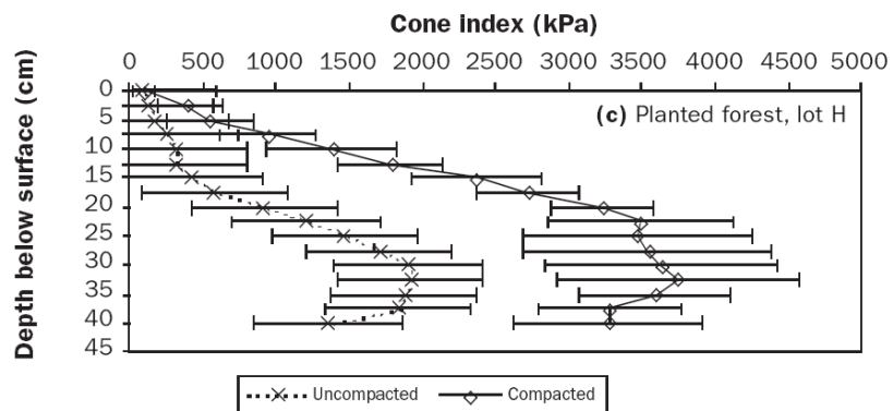
Figure 3: Soil compaction plot showing a consistent increase in Cone Index (compaction) and a larger increase near the bottom of the soil profile in a wooded site that was cleared for development (Gregory, Dukes, Jones, 2006).
