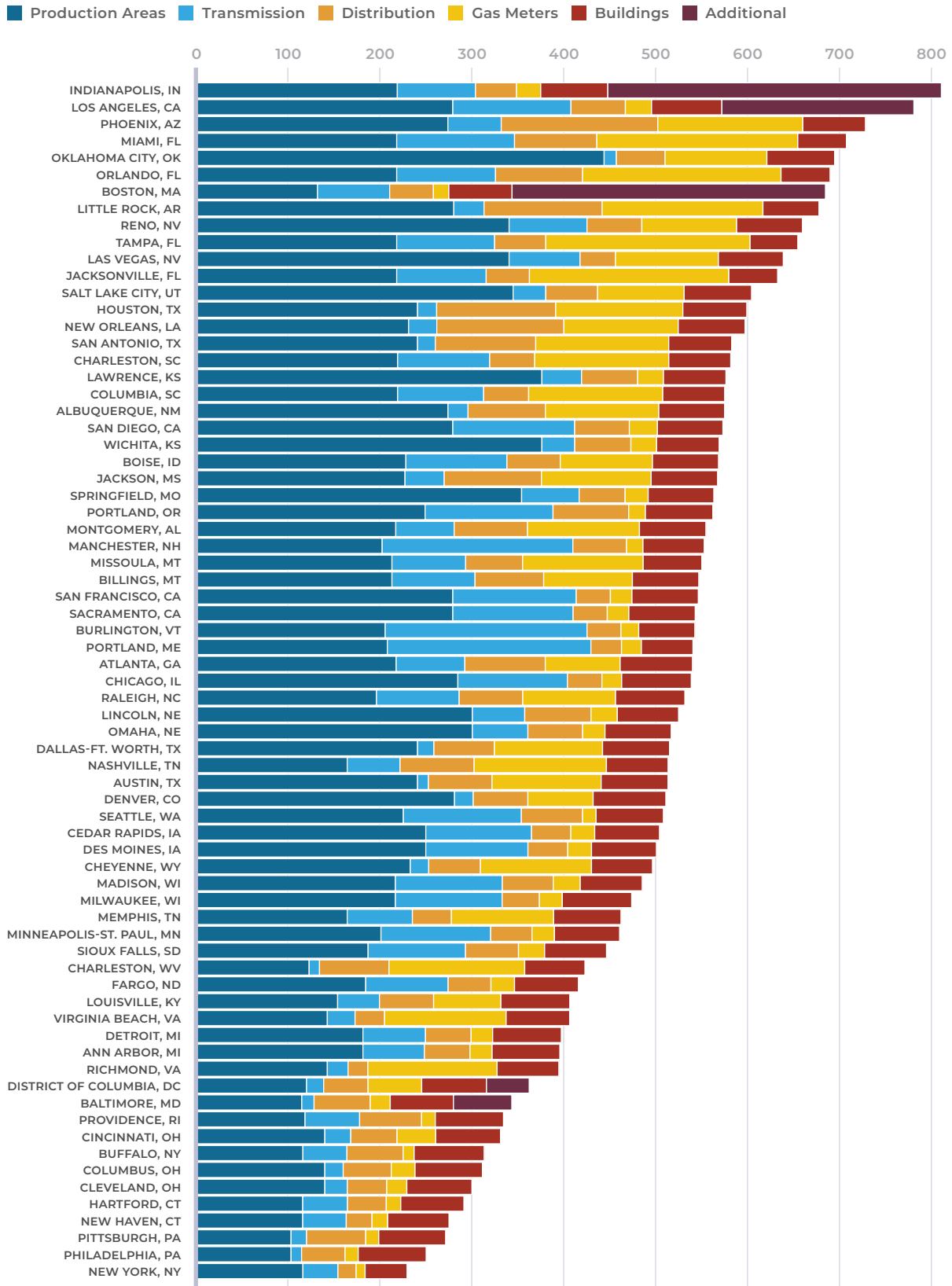
FIGURE 1. Gas Index results for the rate of life cycle methane leakage for the gas supplies for the 71 cities evaluated.
