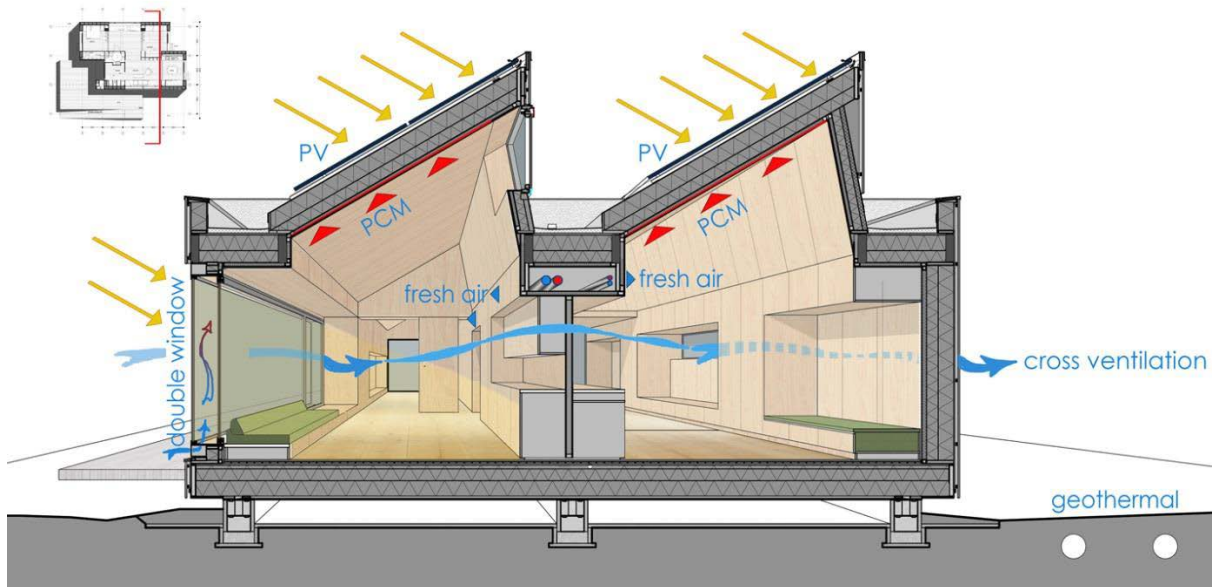
Fig. 1.10. A section of the building that shows the interaction and operation of the strategies applied (Finocchiario et al. 2014).
