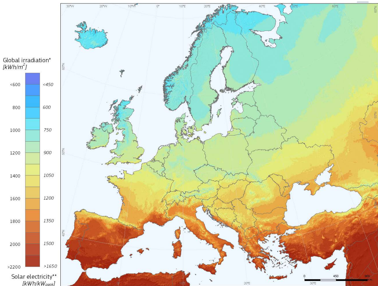
Fig. 1.1. Photovoltaic solar energy potential in European countries (PVGIS 2012).
