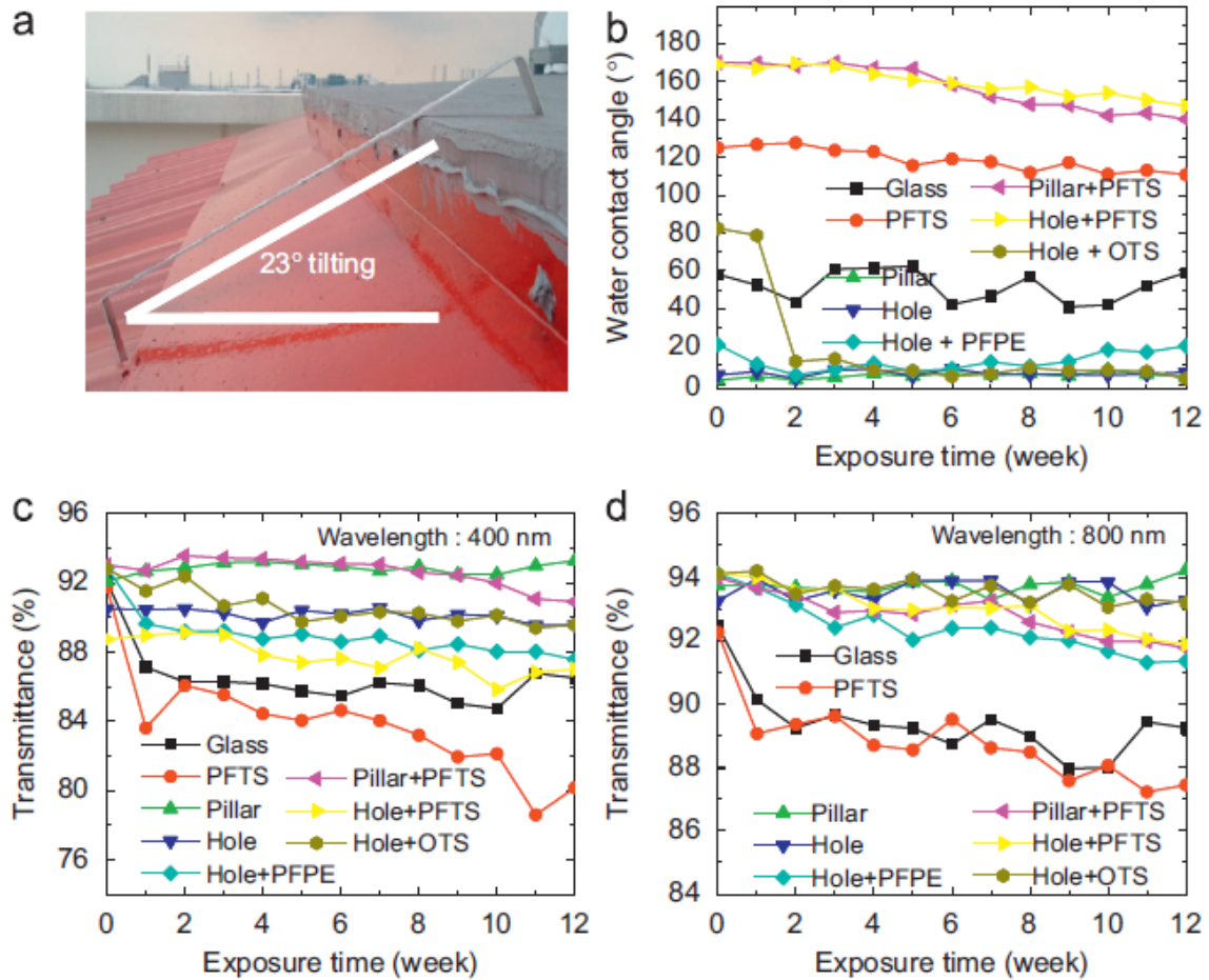
Fig. 4.14. (a) Tilting angle of photovoltaic devices in outdoor test. (b) Exposure time (week) versus water contact angle ( ^\circ ) for different surface coatings. (c) Exposure time (week) versus transmittance (%) for different surface coatings at wavelength 400 nm. (d) Exposure time (week) versus transmittance (%) for different surface coatings at wavelength 800 nm.
