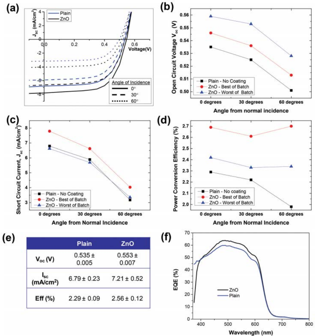
Fig. 4.25. (a) J–V characteristics of NW solar cells, (b) open circuit voltage, (c) short circuit currents and (d) efficiencies of the cells at various incidence angles of light. Note the efficiencies are corrected for light intensity change with tilt, (e) table showing average values and standard deviation for the samples measured and (f) comparison of the external quantum efficiency (EQE) of representative samples (Hiralal et al. 2014).
