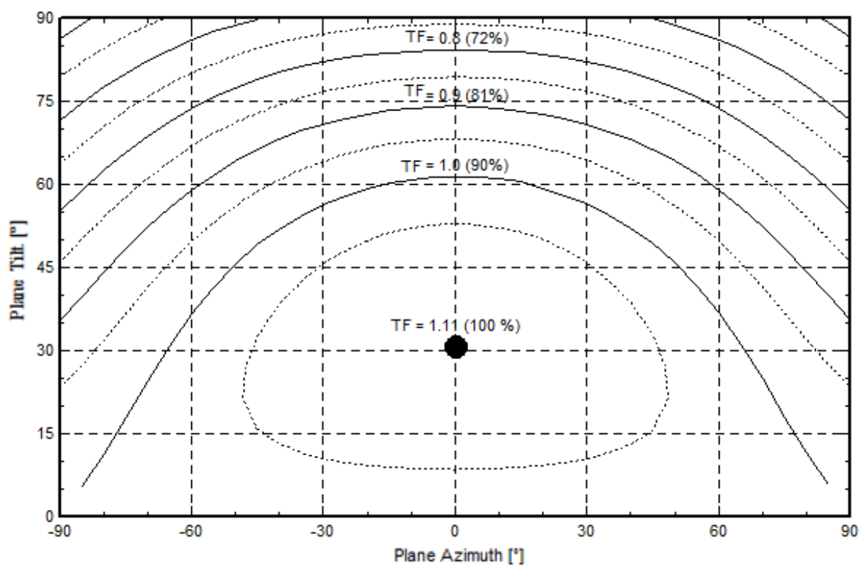
Fig. D.2. Transposition factor variation as function of plane tilt and plane azimuth. Values during the summer for Oslo (plotted by the author through PVsyst).
