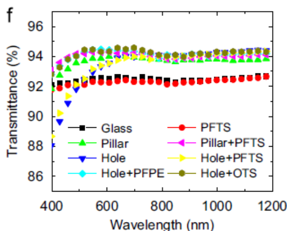
Fig. 4.13. Wavelength (nm) versus transmittance (%) for different coatings (pillar, hole, hole+PFPE, PFTS, pillar+PFTS, hole+PFTS, hole+OTS) on glass sample (Son et al. 2011).
