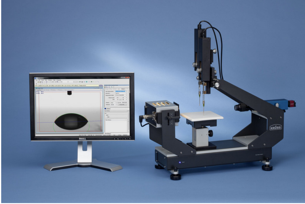
Fig. 4.27. A DSA30 drop shape analysis system from Krüss.
