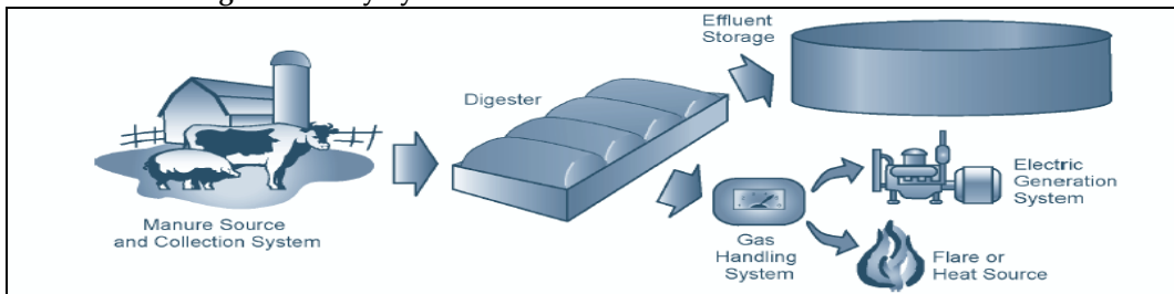
Exhibit 5-5. Biogas Recovery Systems
