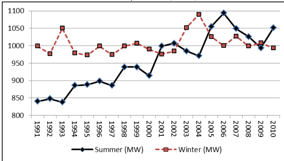
Exhibit 3-4. Vermont Seasonal Peaks, 1991–2010 (in MW)
