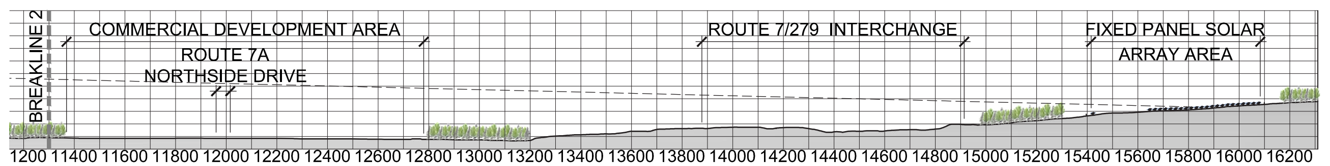
CROSS-SECTION A - SOUTHERN VERMONT COLLEGE THROUGH PROJECT SITE - ENLARGEMENTS
