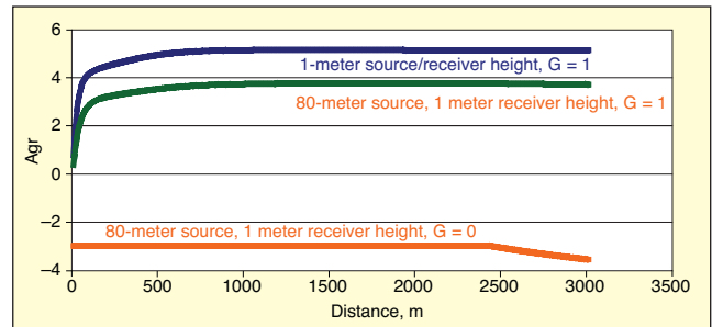
Figure 1. Spectral ground attenuation ( A_{gr} ) over distance for an 80-m and 1-m-high source; 1-m-high receiver and ground factor set to 1 (soft) and 0 (hard).
