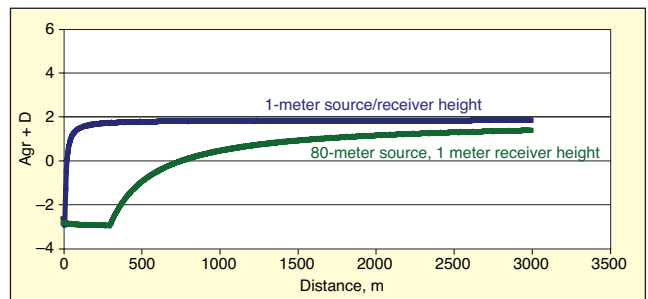
Figure 2. Nonspectral ground attenuation ( A_{gr} + D ) over distance for an 80-m and 1-m source and 1-m receiver height. Nonspectral ground attenuation is not a function of ground hardness.
