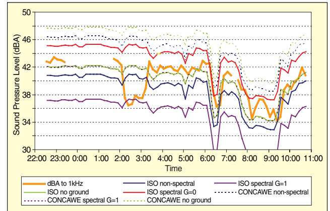
Figure 5. Comparison of monitored sound levels over time at 610 m (shown in orange) with modeled sound levels under various combinations of ground attenuation factors and meteorological factors.
