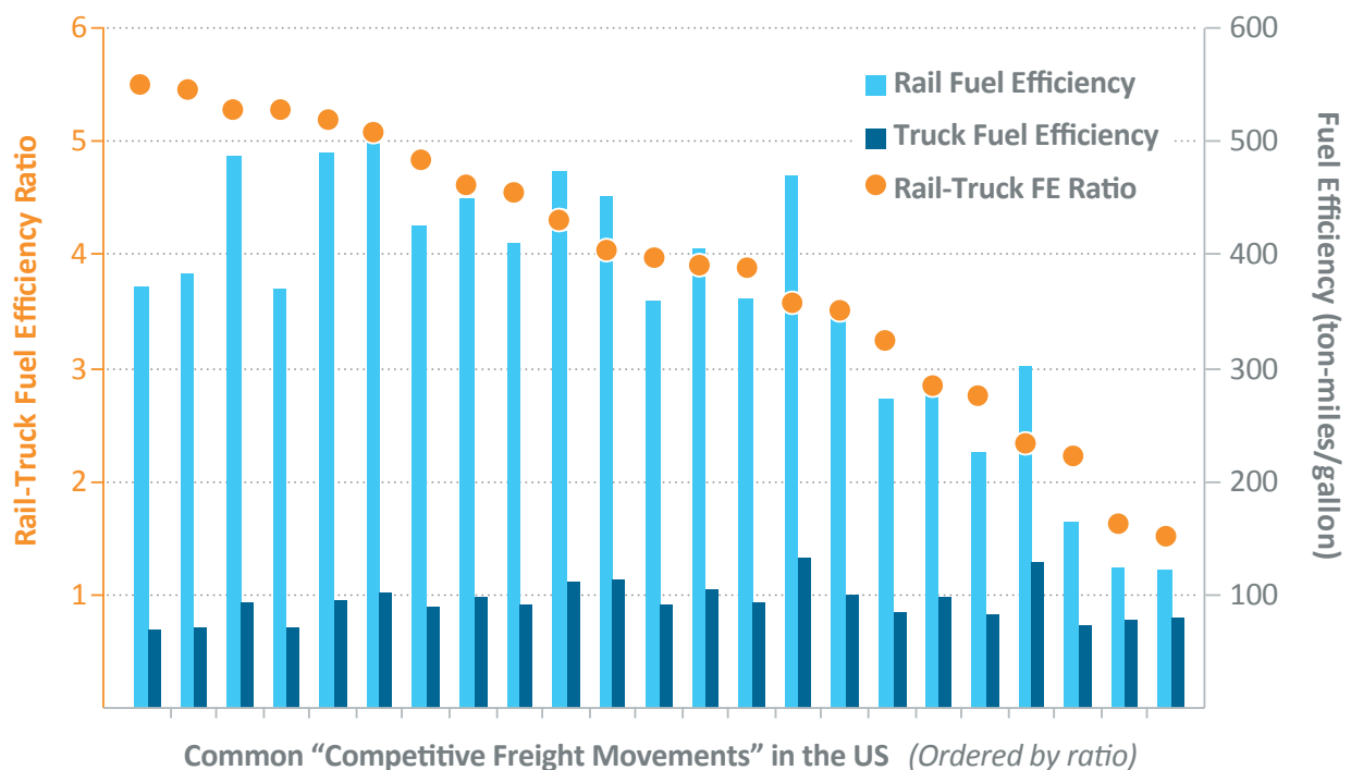
Figure 4.8: Relative Fuel Efficiencies of Freight Movement by Rail Versus Truck
