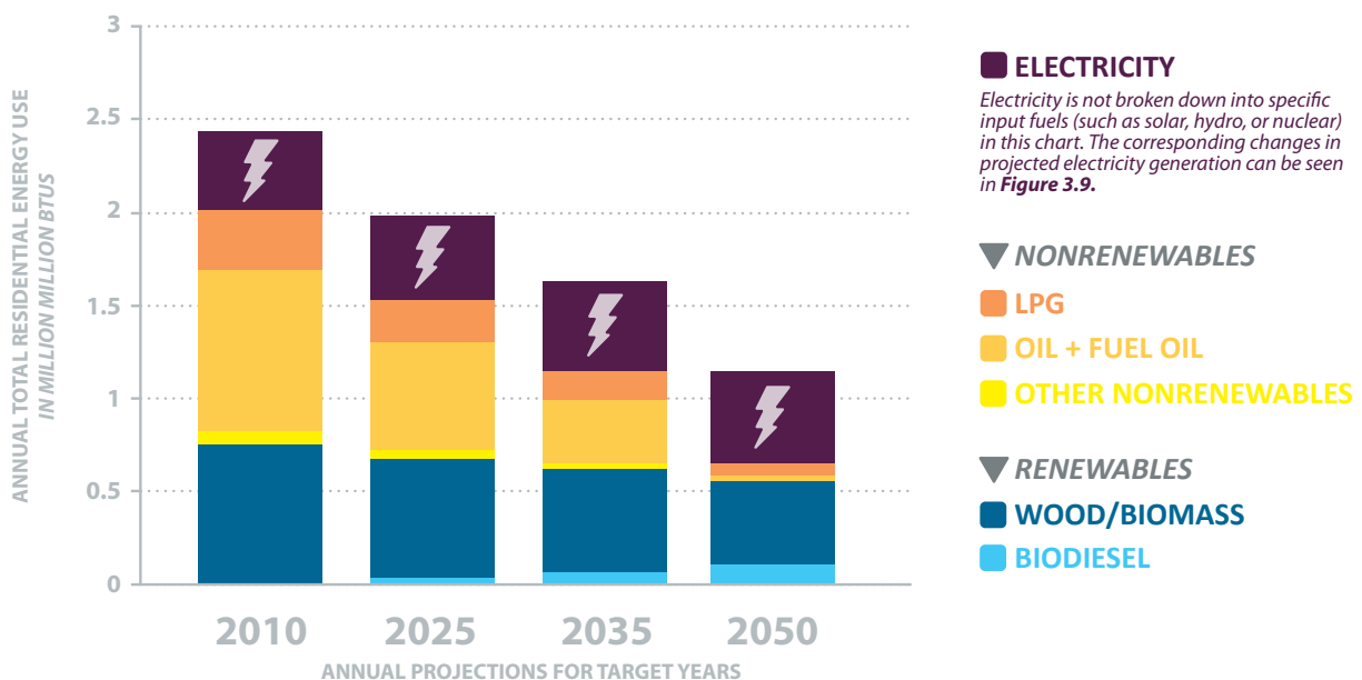
FIGURE 3.3: BENNINGTON REGION—RESIDENTIAL ENERGY USE BY FUEL TYPE, 2010 - 2050
