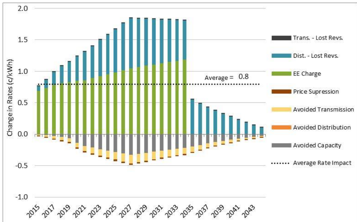
Figure 5.8 BED Business Non-Demand Rate Impacts by Component (c/kWh)
