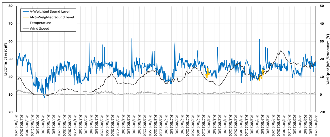
Figure 25. Sound Level and Weather Data: Site C, May 13 – May 20, 2019
