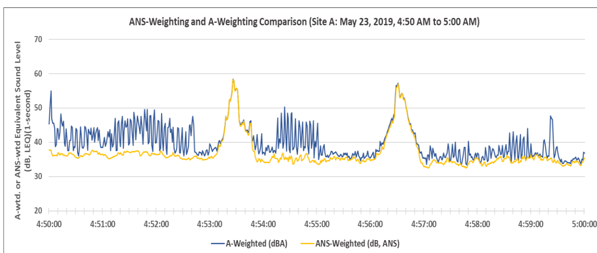
Figure 14. ANS-Weighting and A-Weighting Comparison
