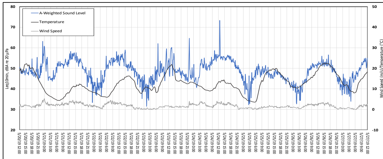
Figure 17. Sound Level and Weather Data: Site A, May 20 – May 27, 2019
