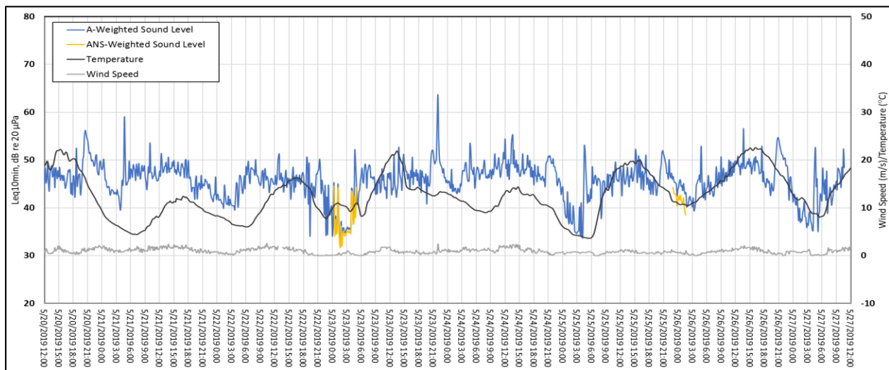
Figure 26. Sound Level and Weather Data: Site C, May 20 – May 27, 2019
